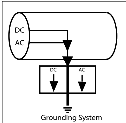
FIGURE 2 "Short Circuit" Mode For Over-Voltage Protection
