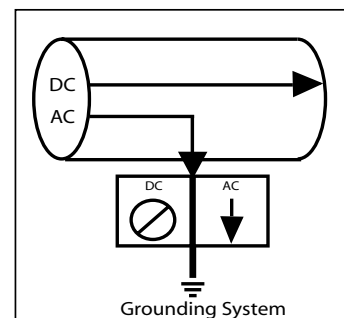
FIGURE 1 The ISP in Normal Mode For Cathodic Isolation
